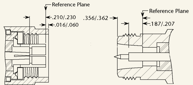
Plug (male)
