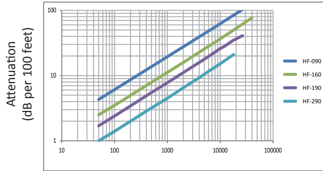
Attenuation vs. Frequency (Typical)
